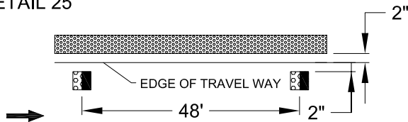
DETAIL 25A- USE ON FREEWAY RAMP AND CONNECTORS
